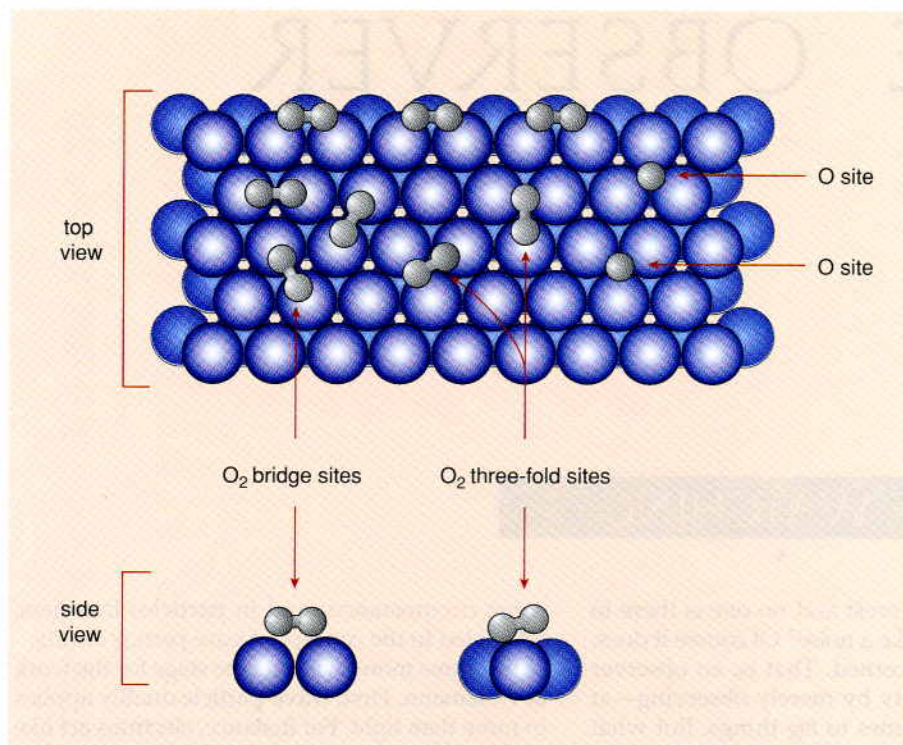
Figure 3. Schematic of O_2 molecules and atoms (gray) adsorbed on a platinum surface (left). The image generated by the scanning tunneling microscope reveals two shapes oxygen molecules chemisorbed onto the platinum surface (right). Molecules can appear "clover-leaf" (B) or "pear-like" (F) shapes. In some places one sees the molecules dissociated to adsorbed oxygen atoms (dark circles marked "o"). (Photograph courtesy of Wilson Ho, reprinted from Stipe et al. with permission from the Journal of Chemical Physics .)
