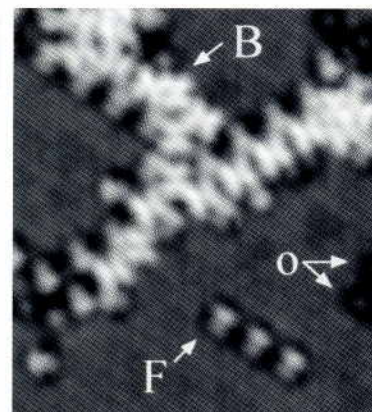
Figure 3. Schematic of O_2 molecules and atoms (gray) adsorbed on a platinum surface (left). The image generated by the scanning tunneling microscope reveals two shapes oxygen molecules chemisorbed onto the platinum surface (right). Molecules can appear "clover-leaf" (B) or "pear-like" (F) shapes. In some places one sees the molecules dissociated to adsorbed oxygen atoms (dark circles marked "o"). (Photograph courtesy of Wilson Ho, reprinted from Stipe et al. with permission from the Journal of Chemical Physics .)
