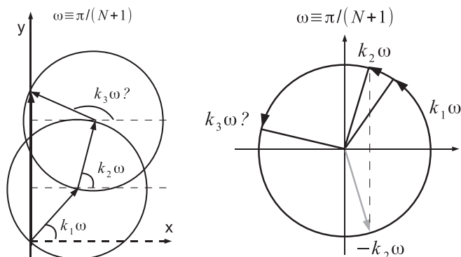
FIG. 2. Left: \cos\left(\frac{k_1\pi}{N+1}\right) + \cos\left(\frac{k_2\pi}{N+1}\right) + \cos\left(\frac{k_3\pi}{N+1}\right) = 0 is equivalent to the phasors adding to a vertical vector. The circles shown are unit circles. Right: Vanishing sums of roots of unity imply vanishing sums of cosines on the upper half plane since one can reflect any phasor without changing the cosine.
