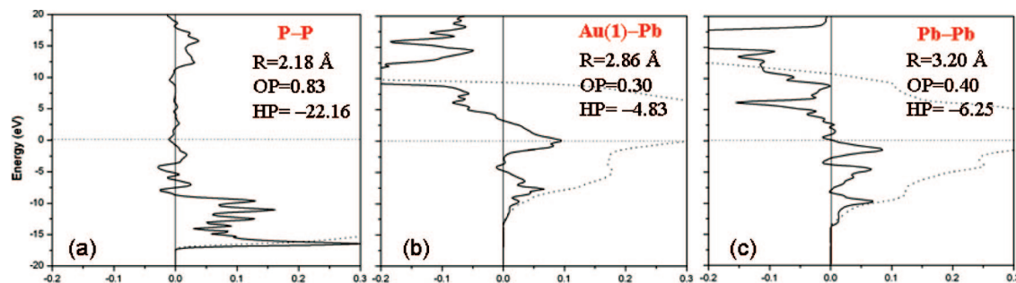
Figure 3. Crystal orbital overlap population (COOP, eH method) curves for bonds in \text{Au}_2\text{PbP}_2 . The corresponding distances as well as the OP and HP values are listed (integrated up to the Fermi level). The solid line represents the COOP curve, while the dotted line represents the integration. The dotted horizontal line indicates the adjusted Fermi level at 0 eV.
