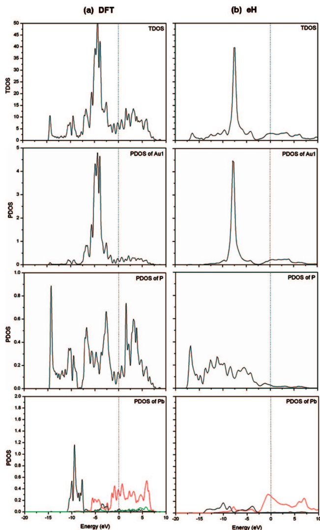
Figure 2. (a) Calculated density of states (DOS) of Au 2 PbP 2 (DFT). (b) Calculated DOS of Au 2 PbP 2 (eH). The dotted vertical line indicates the adjusted Fermi level at 0 eV. The combined (s + p + d) partial or projected (PDOS) of one P and Au1 atom are shown. The PDOS of Au2 is very similar to the PDOS of Au1. For one Pb atom, the s, p, and d orbital contributions to the DOS are given separately by black, red, and green lines, respectively. Note that the PDOS scales are different for each element.
