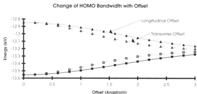
Figure 5. Change of the HOMO bandwidth with longitudinal and transverse offsets for the ethylene molecule.
