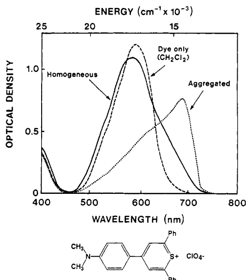
Figure 12. Aggregation and concomitant broadening of the absorption spectra of thiopyrylium dyes occurs in concert with a 100-fold increase in photosensitivity. Reprinted with permission from ref 34. Copyright 1978 American Institute of Physics.
