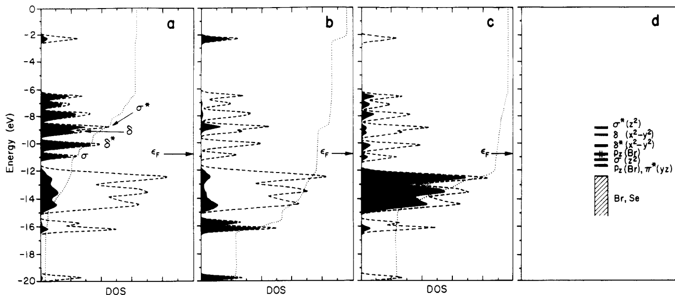
Figure 6. Total DOS (dashed line) and projected DOS (blackened area) for \text{NbSe}_2\text{Br}_6 giving (a) the Nb, (b) the Se, and (c) the Br contributions. The energy levels of a molecular [\text{Br}_3\text{NbSe}_2\text{Br}_2\text{NbBr}_3]^{2-} unit are shown in (d).
