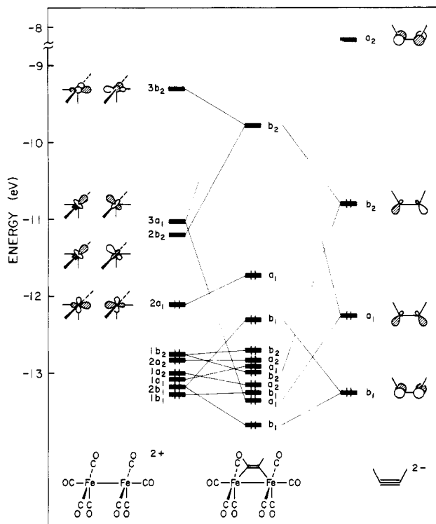
Figure 8. The interaction of (\text{CO})_4\text{FeFe}(\text{CO})_4^{2+} with \text{C}_2\text{H}_2^{2-} . The Fe-Fe distance is 2.8 Å and the \text{C}_{\text{ac}}-\text{C}_{\text{ac}}-\text{H} angle is 120^\circ .
