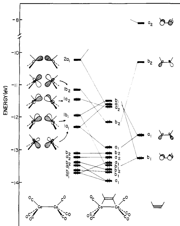
Figure 4. The orbitals of \text{Co}_2(\text{CO})_6(\mu\text{-C}_2\text{H}_2) in the parallel bonding mode.
