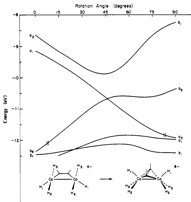
Figure 11. Correlation diagram for the interconversion of the model system \text{Co}_2\text{H}_6(\mu\text{-C}_2\text{H}_2)^{6-} from the A-frame geometry to the "linear spine" geometry. The rotation angle of acetylene is indicated with 0^\circ taken as parallel and 90^\circ perpendicular. The \text{Co-C}_{ac} distance was kept constant at 2.0 \text{ \AA} for the entire motion. Perpendicular geometry includes angles \text{Co-Co-H}_1 = 152^\circ and \text{C-C-H} = 140^\circ .
