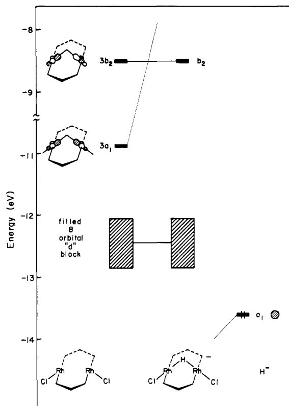
Figure 4. Orbital scheme of the model for a \mu -H A-frame, \text{Rh}_2(\mu\text{-H})\text{Cl}_2(\text{dpm}')_2^- .
