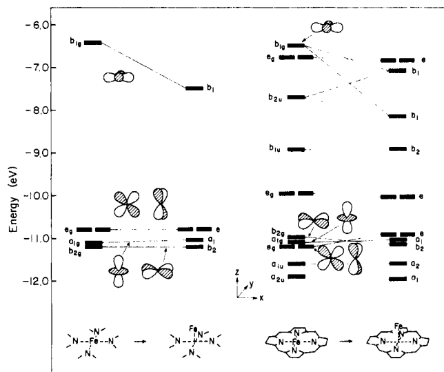
Figure 1. Levels of Fe(porphyrin) and its model compound \text{Fe}(\text{NH}_2)_4^{2-} . The right half of the figure shows the levels of Fe(porphyrin) and the left half shows those of \text{Fe}(\text{NH}_2)_4^{2-} . From left to right in each half: the Fe atom sits in the middle of the porphyrin or (\text{NH}_2)_4 plane; Fe moves up by 0.5 Å out of the plane.
