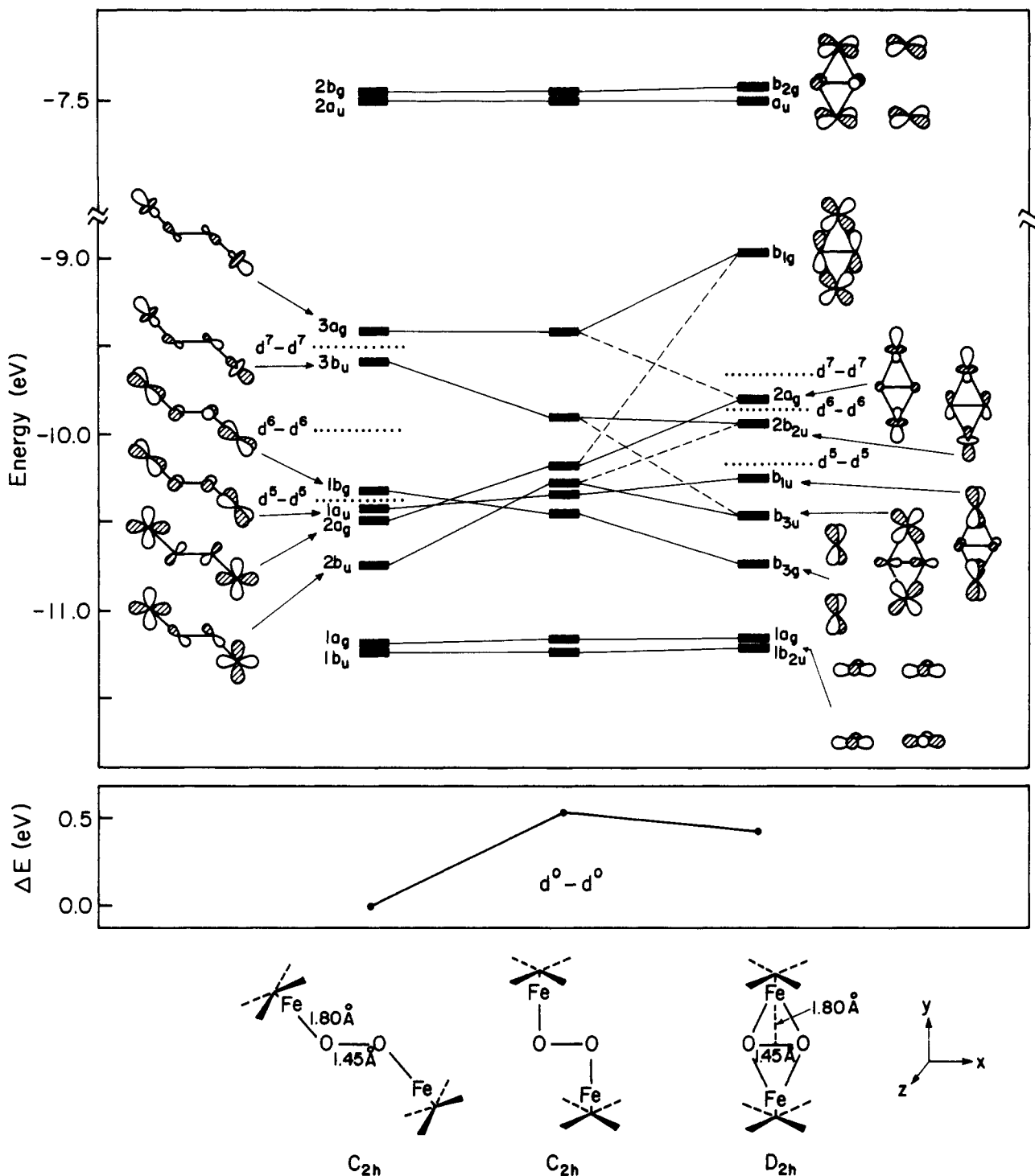
Figure 7. Top: Orbital correlation diagram for the deformation of N_4Fe-O-O-FeN_4 linking the two trans bent geometries, angle Fe-O-O = 120^\circ and 90^\circ , and the side-on structure. The O_2 fragment is staggered with respect to N atoms of both N_4 units. Dotted lines and d^n-d^n labels indicate the filled-unfilled level gap for various d electron counts. Bottom: total energies for the d^0-d^0 electron configuration of the three geometries.
