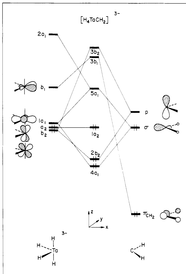
Figure 1. Diagram to show the interaction of the frontier orbitals of \text{H}_4\text{M} with those of \text{CH}_2 in [\text{H}_4\text{TaCH}_2]^{3-} .
