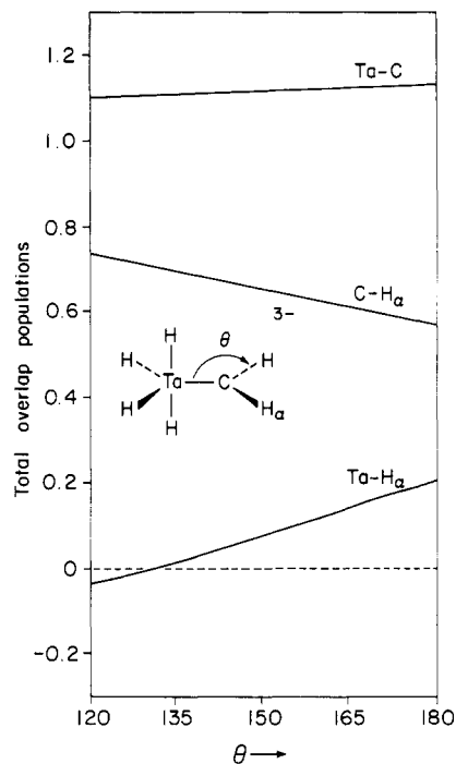
Figure 3. Total overlap populations in the triad, Ta-C, C- H_a , and Ta- H_a , as a function of \theta .
