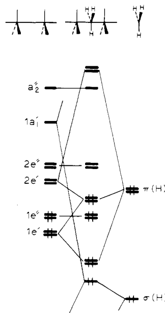
Figure 10. Interaction diagram for H_3M_2L_8 in conformation 44 . The electron count shown is for a d^4 dimer.
