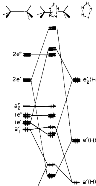
Figure 8. Construction of the orbitals of H_5M_2L_6 .
